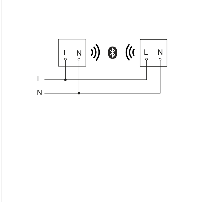
Master/master interconnection circuit diagram
